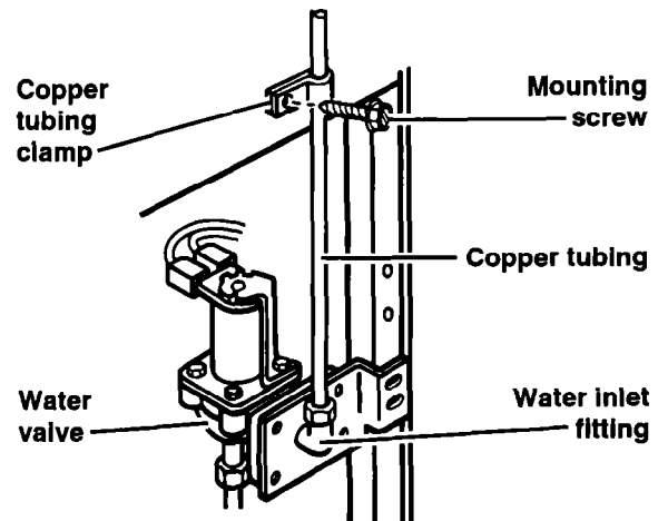
Style #1 valve
